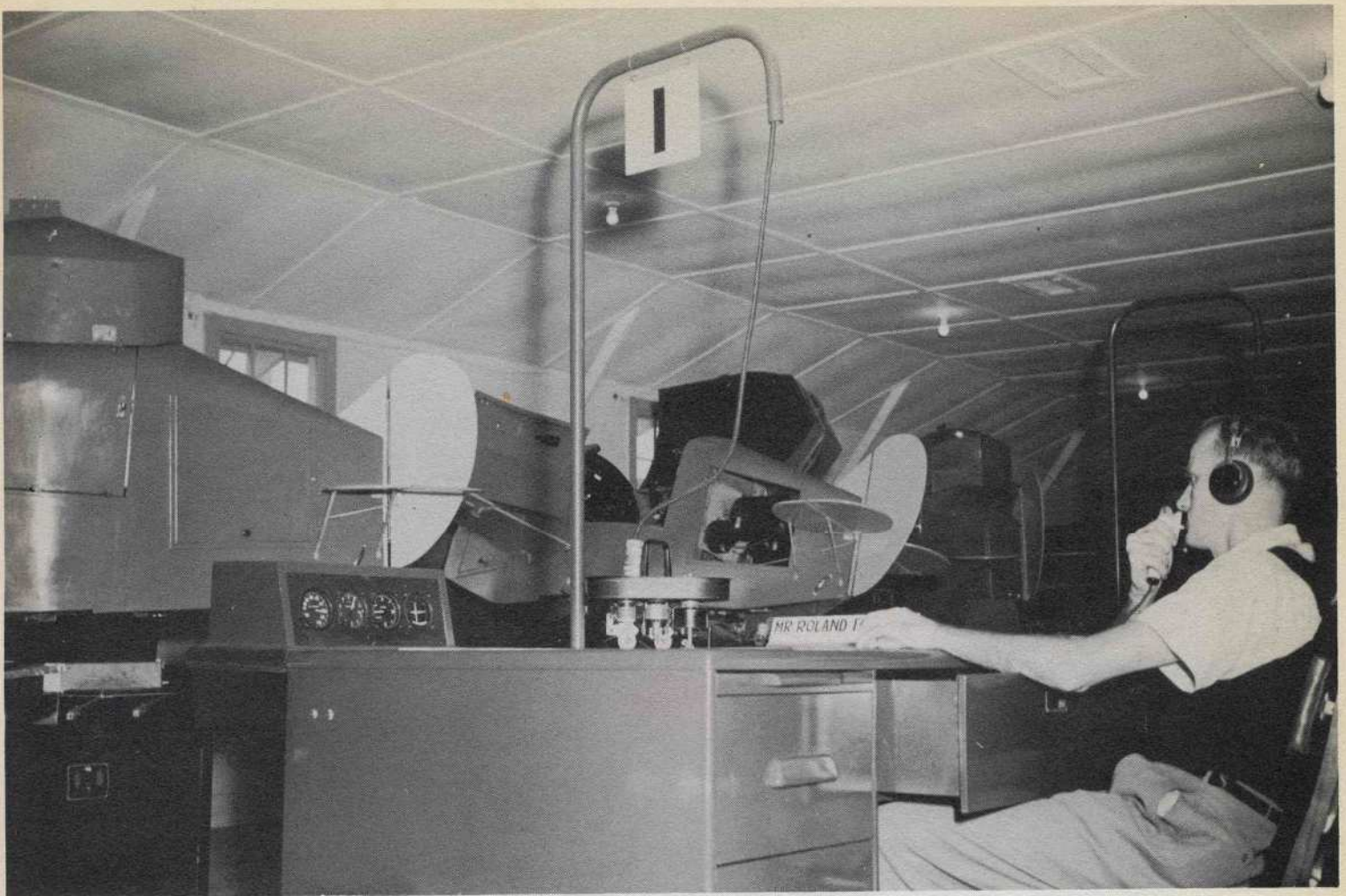
The AN T-18 Instrument Trainer
